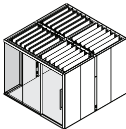
CD05 Corner Glass Front, Right Hand Door Understanding ▶ Page 20 Specifying ▶ Page 102
